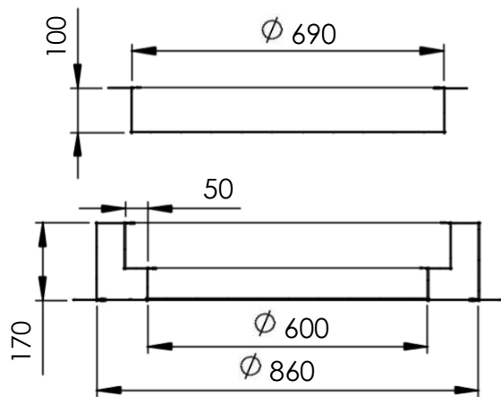
SECTION C-C SCALE 1 : 15
